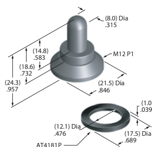
AT4181
